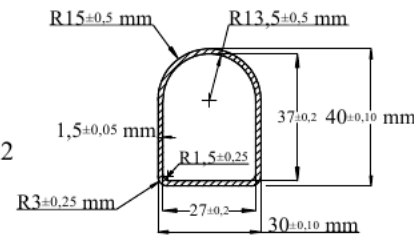
COLLECTOR DETAIL : 5:1
