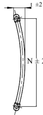
COLLECTOR DETAIL : 5:1
